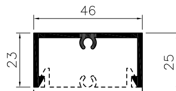
HORIZONTAL
