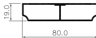
BARROTE
