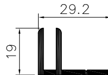
SUPPORT LAME
