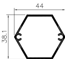
BARREAU EXAGONALE GRAND
