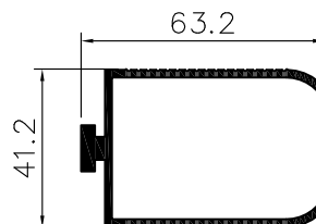
PROFILE UNION CENTRAL
